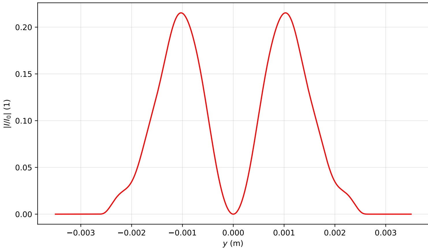
Intensity profile I(x = 0, y, z = 3.742)/I_0 , P_{in}=1.0P_{cr} , artificial time
